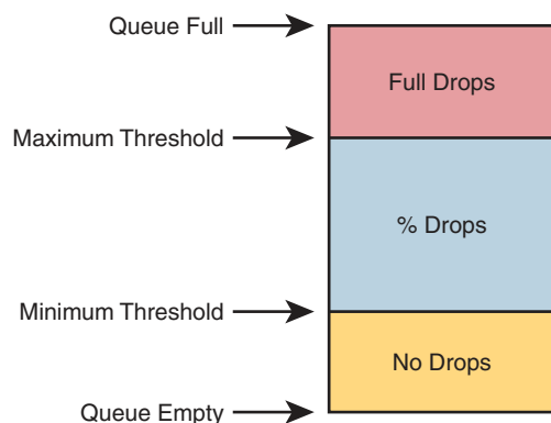
Figure 11-23 Mechanisms of Congestion Avoidance
