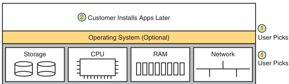
Figure 15-9 IaaS Concept
