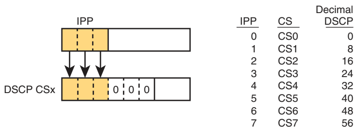
Figure 11-12 Class Selector
