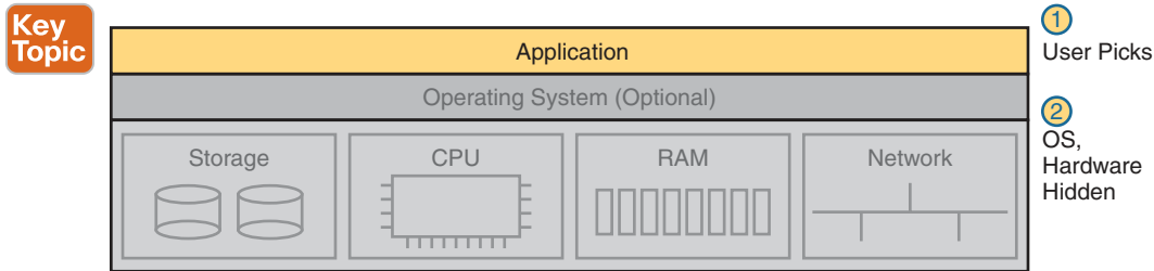
Figure 15-11 SaaS Concept
