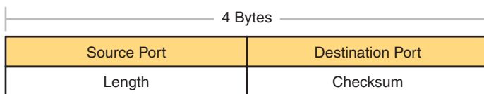
Figure 1-10 UDP Header
