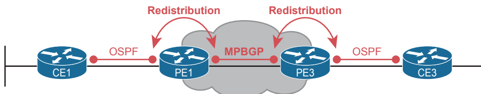
Figure 14-15 MPLS VPN Using Redistribution with MPBGP at PE Router
