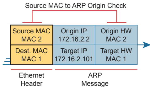
Figure 8-14 DAI Filtering Checks for Source MAC Addresses
