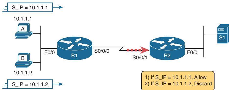
Figure 2-2 Pseudocode to Demonstrate ACL Command-Matching Logic
